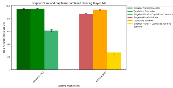
Figure D.1: Results showing the performance of the two combined steering mechanisms, alongside their non-combined mechanisms. With the conceptor-based mechanisms on the left and the point-based mechanisms on the right.
