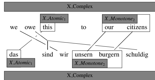
Figure 3: Example of a labeled Hiero rule X\_Complex \rightarrow \langle we\ owe\ X\_Atomic_{\square} \text{ to } X\_Monotone_{\square}, X\_Atomic_{\square} \text{ sind wir } X\_Monotone_{\square} \text{ schuldig} \rangle extracted from the Complex example in Figure 2 by replacing the phrase pairs \langle this, das \rangle and \langle our\ citizens, unsem\ burgern \rangle with (labeled) variables.
