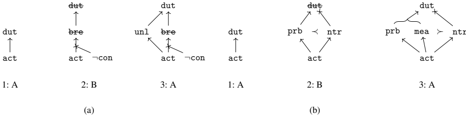
Figure 1. Unpacking (a) a compression rationale and (b) resolution rationale
