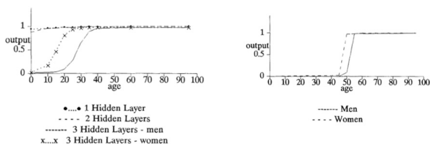
Fig. 12 Neural networks and open texture [Bench-Capon, 1993]
