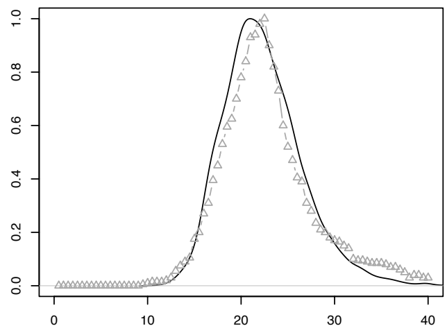
Figure 5. Data (triangles) and model (line) for 21 seconds
