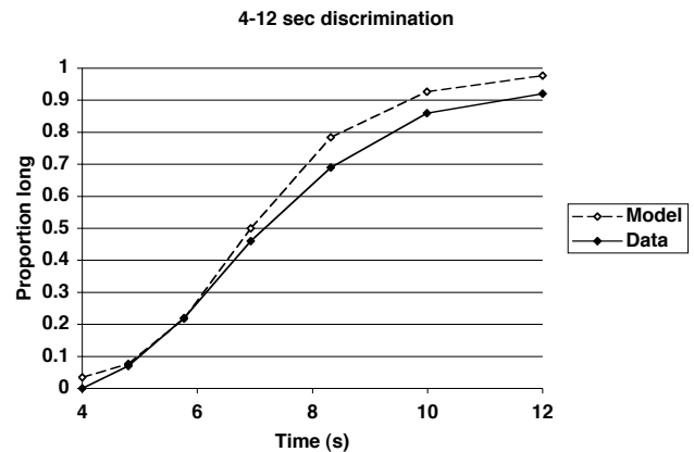
Figure 8. Proportion of "long" responses for intervals between 4 and 12 seconds
